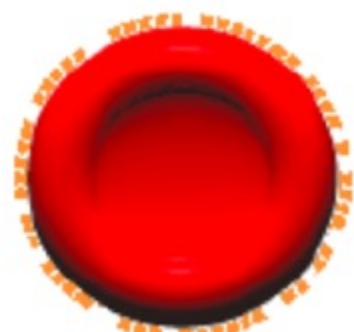
A 2 -Erythrocyte 160'000- 440'000 Antigens
