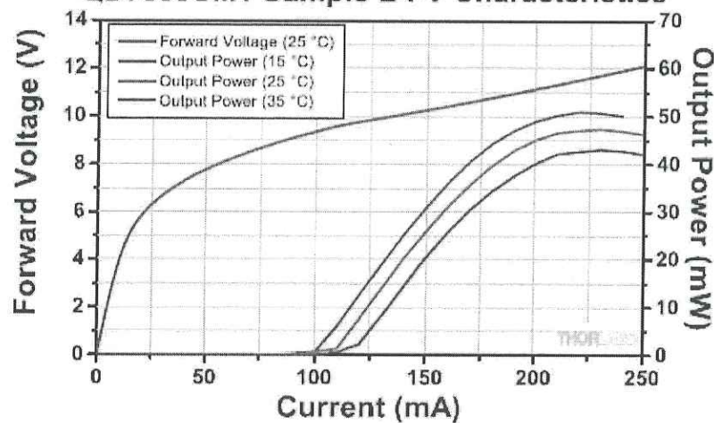
QD7500CM1 Sample L-I-V Characteristics
