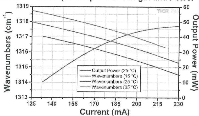
QD7500CM1 Sample Output Wavelength and Power
